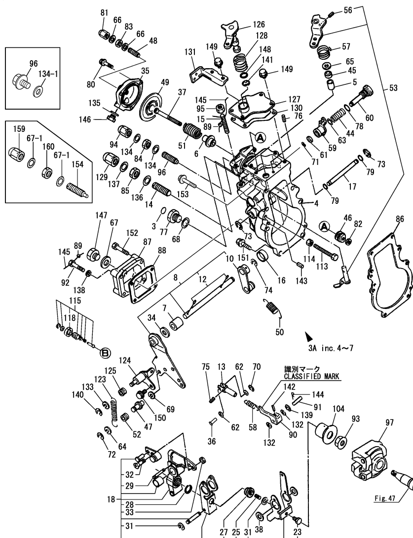
Fig.53. GOVERNOR(4LH-STE)
