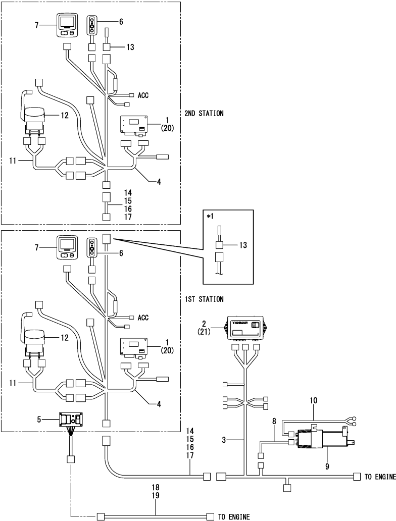
Fig.80. (58C)VC10(SINGLE ENGINE)(OPTIONAL)
