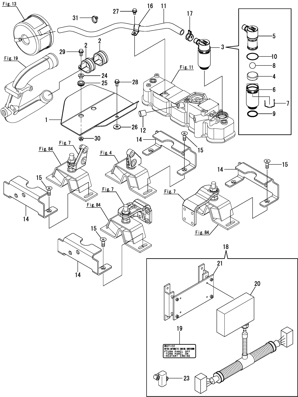
Fig.90. (5A)BREATHER(SOLAS SPEC.)(OPTIONAL)
