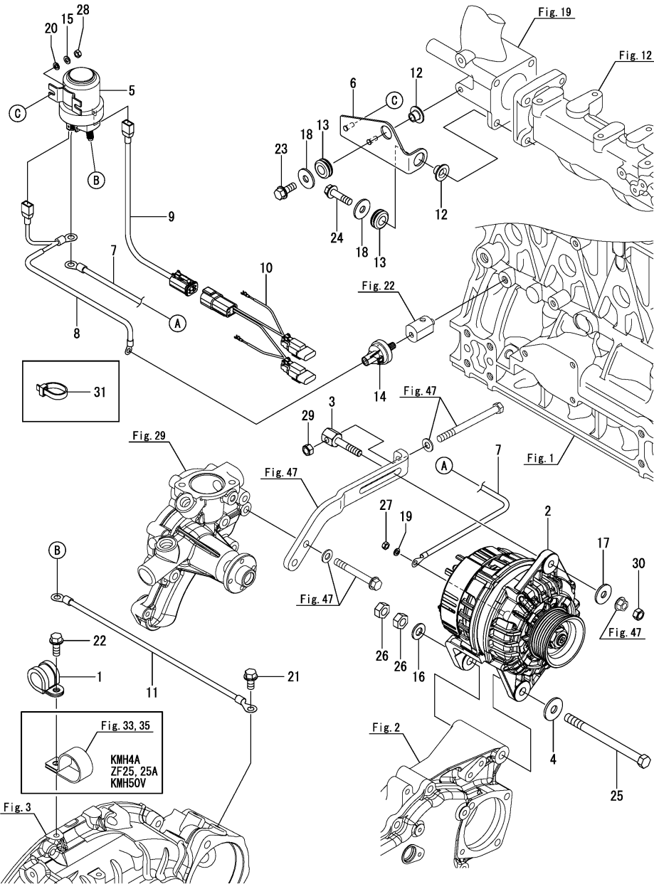
Fig.69. (47A)ALTERNATOR(EARTH FLOAT TYPE REMODEL KIT)(OPTIONAL)
