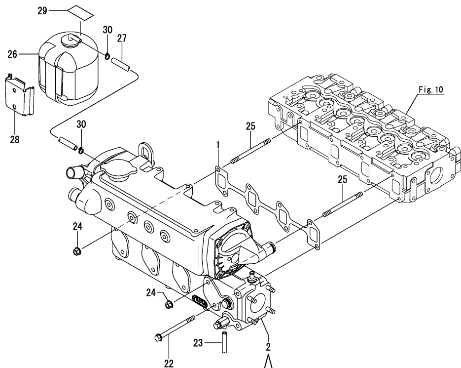
Fig.30. COOLER(FRESH WATER)
