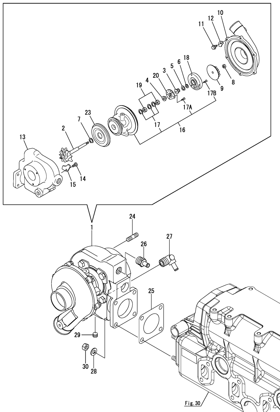
Fig.17. TURBINE
