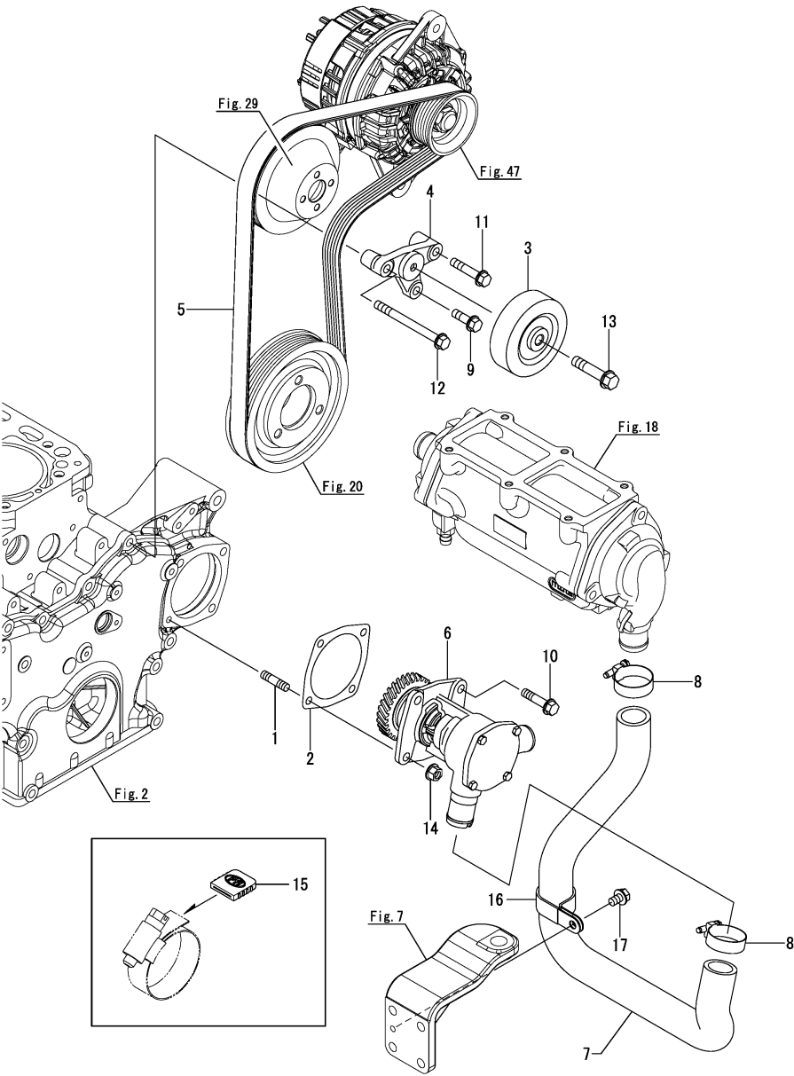
Fig.25. COOLING PUMP(SEA WATER)(FRONT MOUNT SPEC.)
