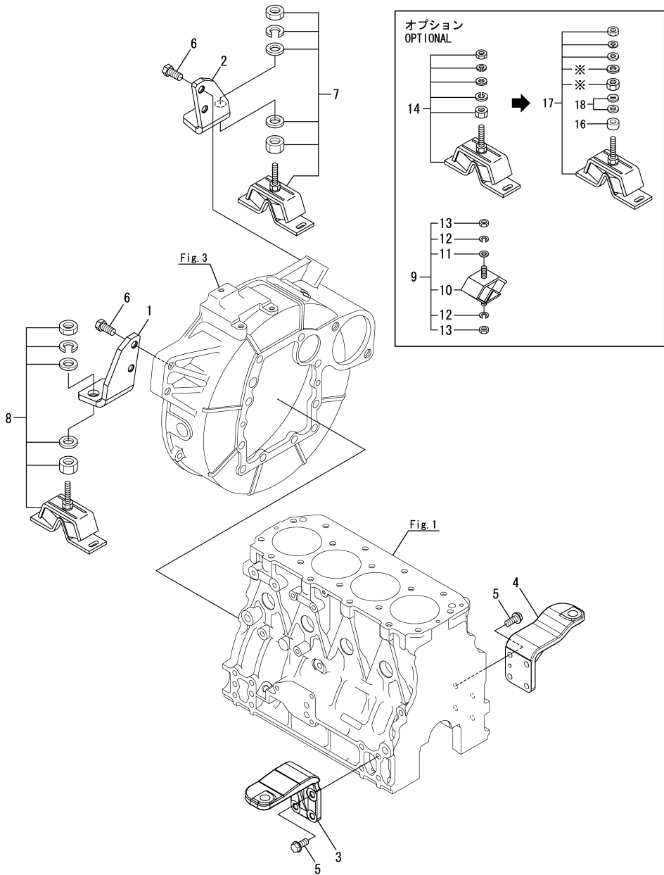
Fig.4. MOUNTING FOOT
