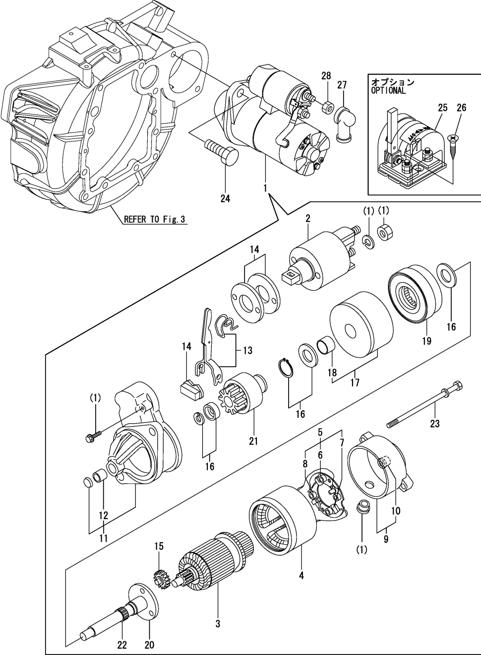
OCR10-M75000 4JH5E Fig.34. STARTING MOTOR
