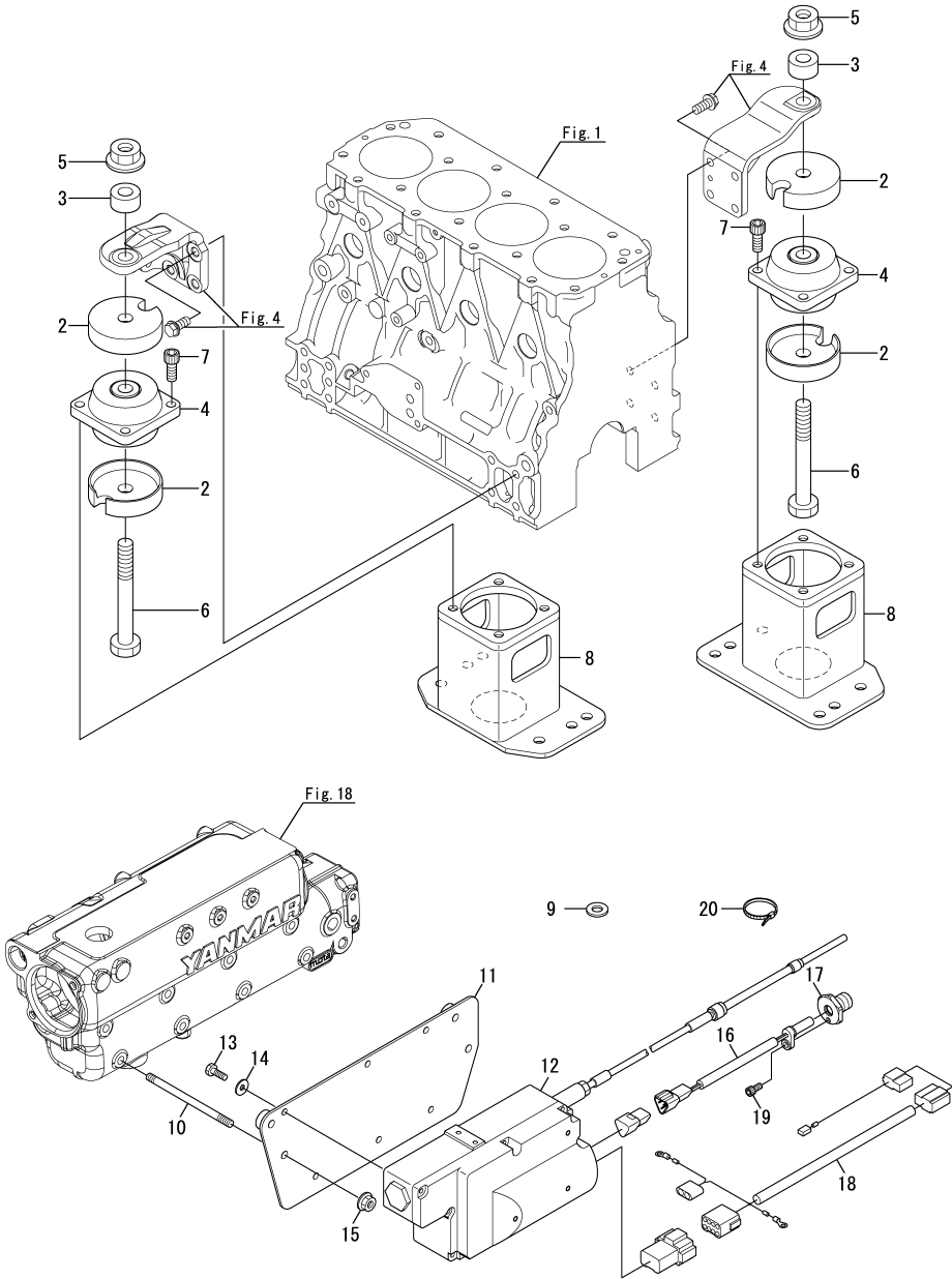
Fig.49. S2 DRIVE(OPTIONAL)
