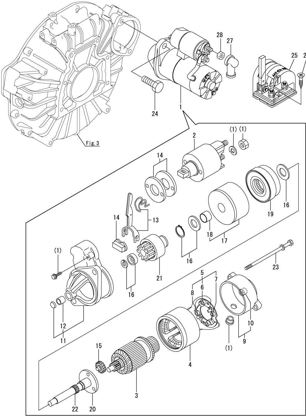
Fig.36. STARTING MOTOR
