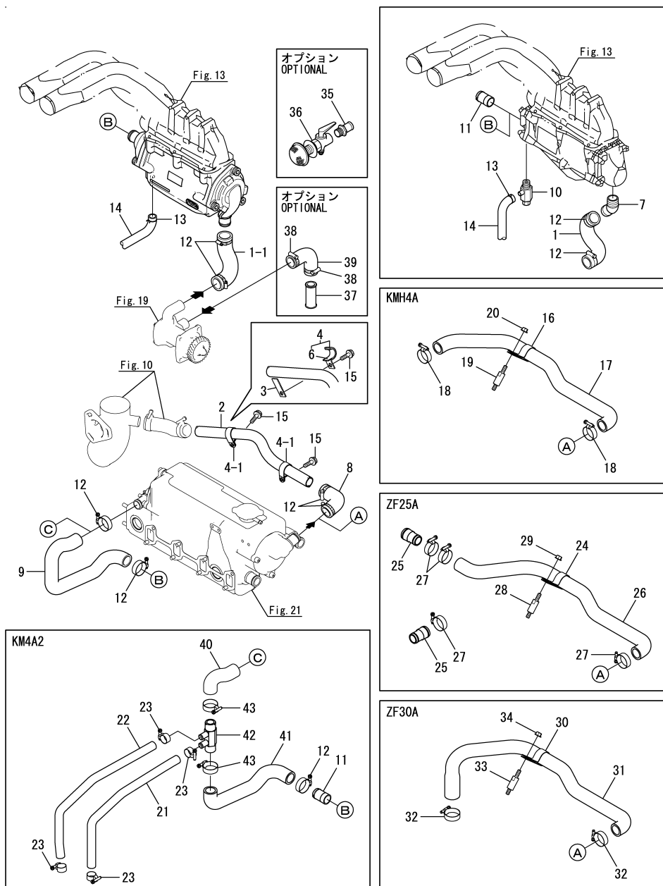
Fig.23. COOLING SEA WATER PIPE(4JH4-HT
