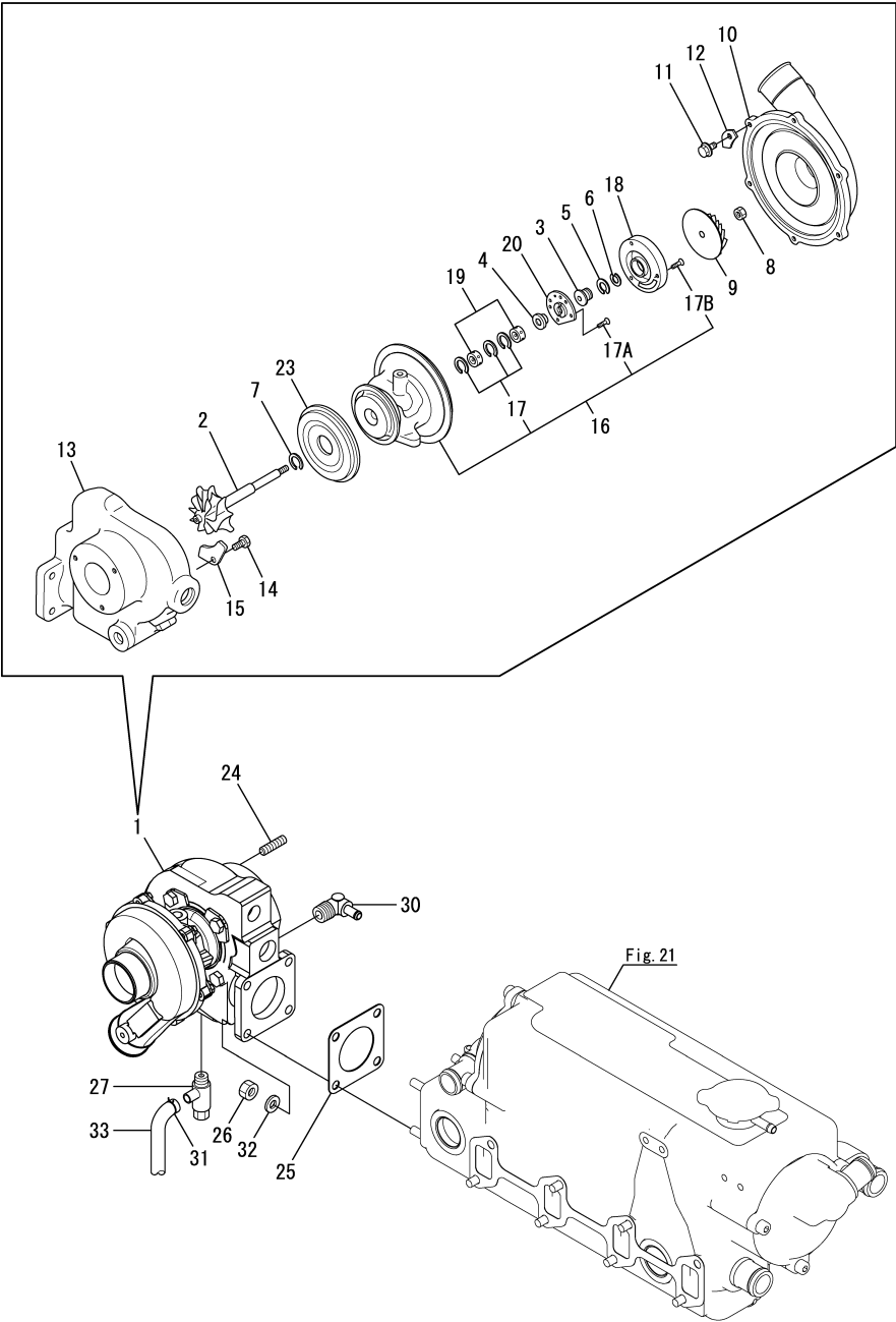
Fig.12. TURBINE(4JH4-HTE/HTE1)
