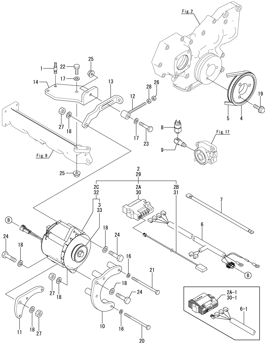
Fig.41. GENERATOR(ADDITION) & GENERATOR MOUNT PART(OPTIONAL)
