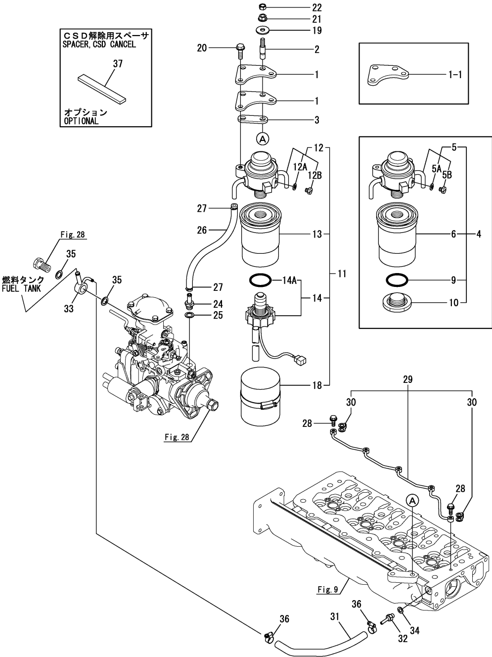
Fig.31. FUEL PIPE & FUEL FILTER
