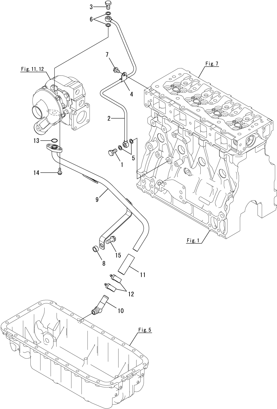
Fig.18. LUB.OIL PIPE
