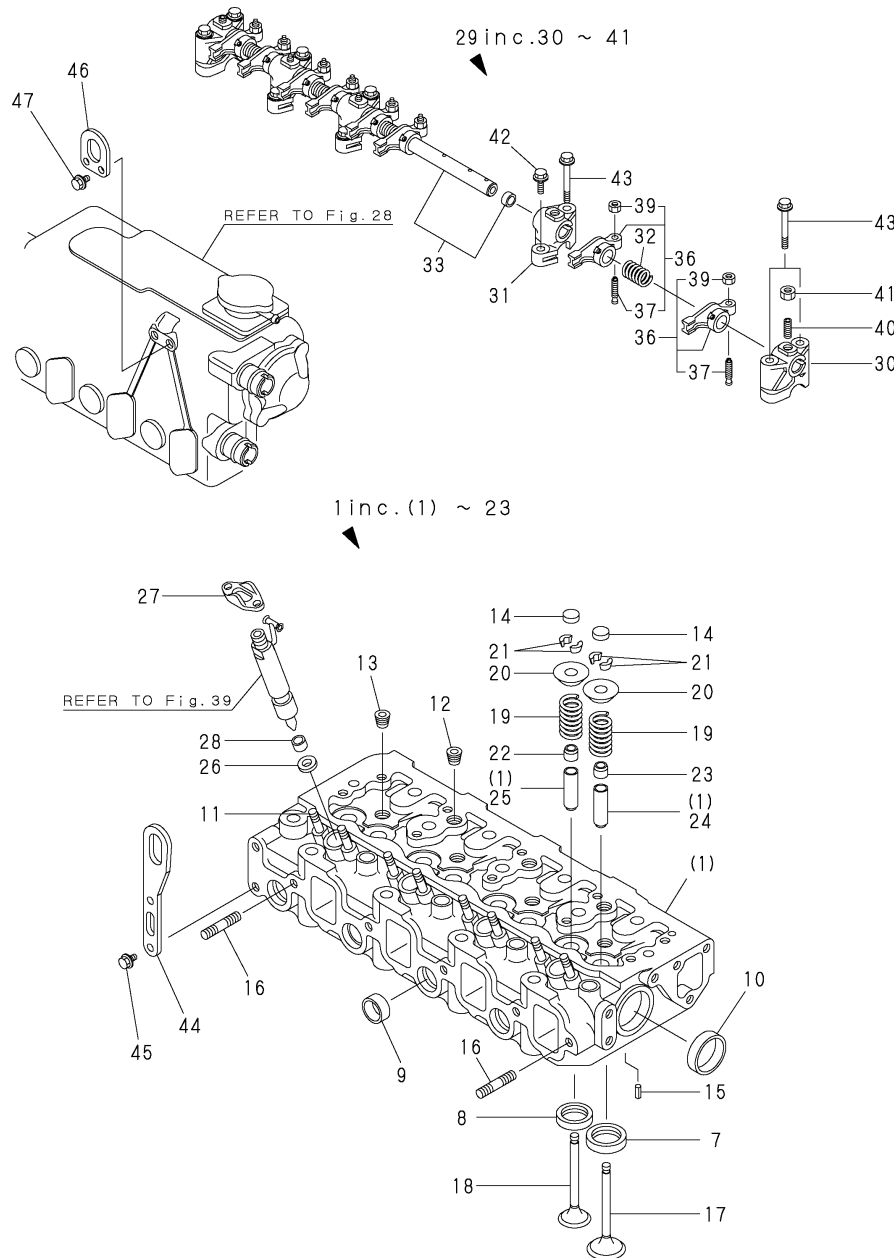
Fig.11. CYLINDER HEAD(4JH3E)
