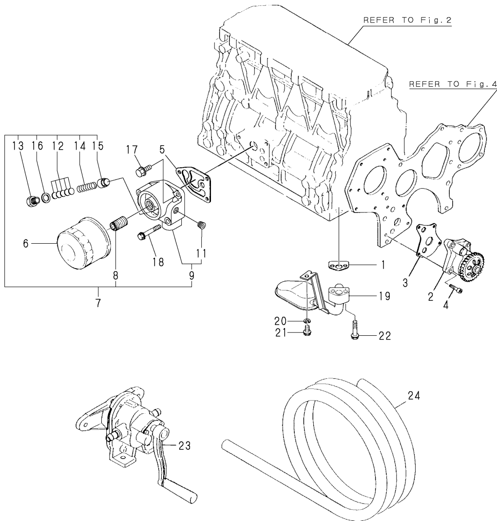
Fig.25. LUB.OIL SYSTEM(4JH3-TE)
