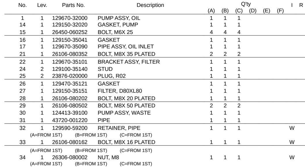
(A)=4JH3E (B)=4JH3CE (C)=4JH3CE1
