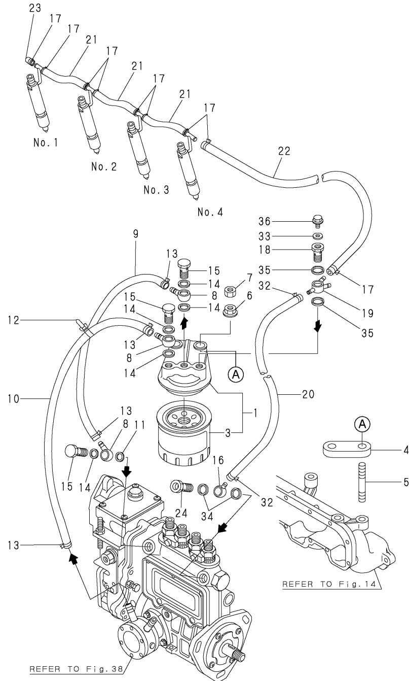
Fig.41. FUEL PIPE(4JH3E)
