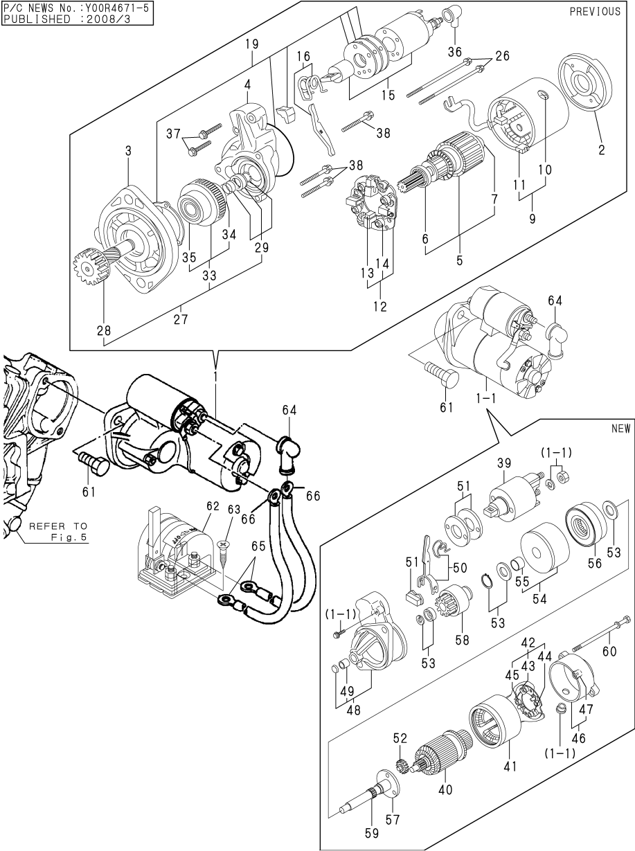
Fig.47. STARTING MOTOR(4JH3-TE)
