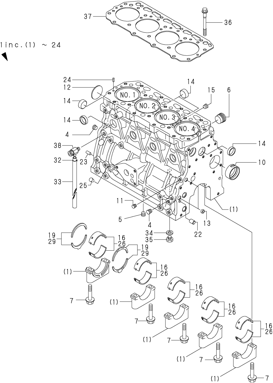
Fig.1. CYLINDER BLOCK(4JH3E)
