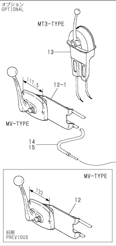
Fig.45. ENGINE STOP DEVIC(4JH3-TE)
