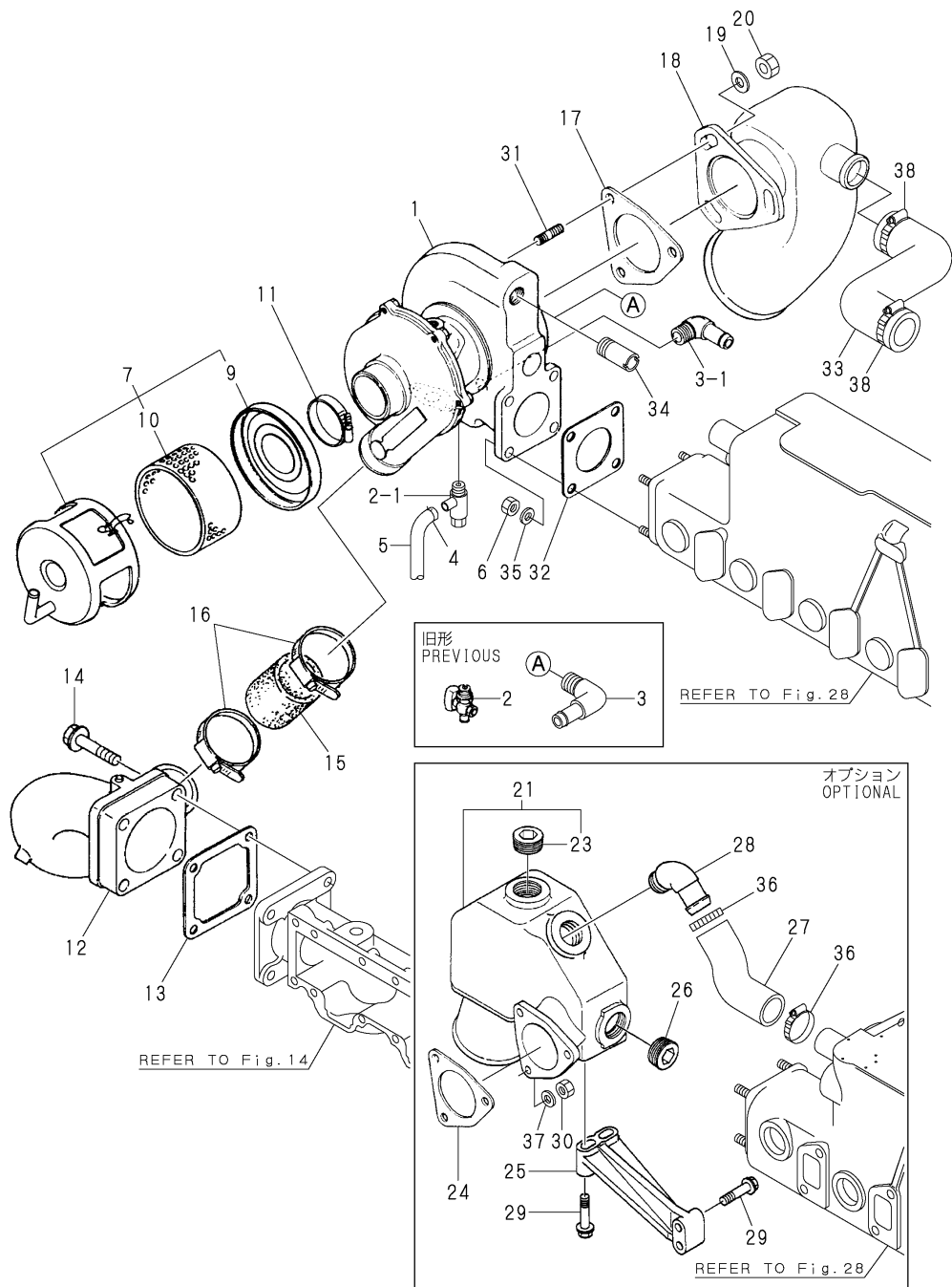
Fig.15. TURBINE
