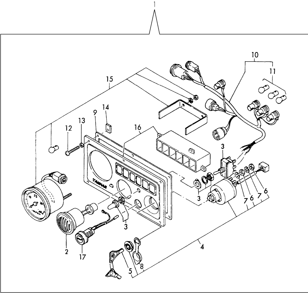
Fig.57. INSTRUMENT PANEL(B:4JH3-TE)
