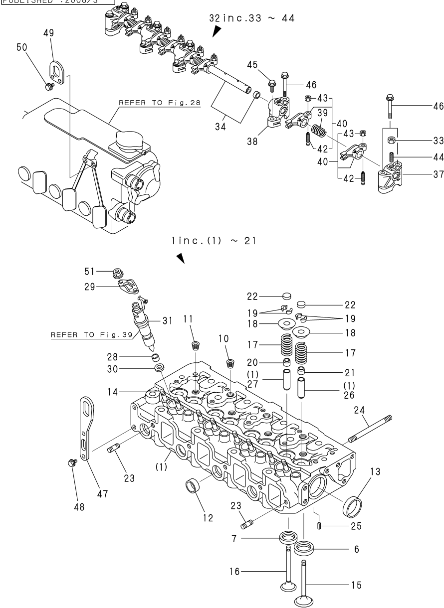
Fig.12. CYLINDER HEAD(4JH3-TE)
