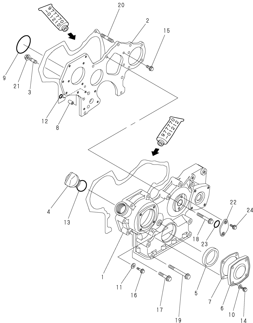
Fig.3. GEAR HOUSING(4JH3E)
